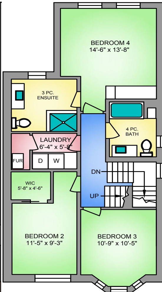
SECOND FLOOR 955 SQUARE FEET
