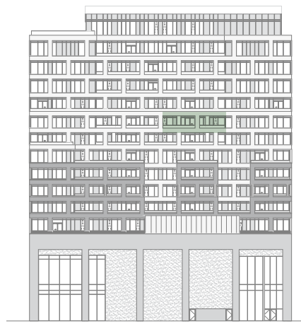
SOUTH ELEVATION
